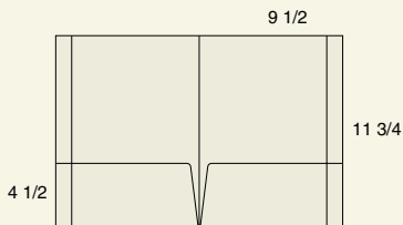
M-200 9 1/2 x 11 3/4 Folder with (2) 4 1/2" glued pockets
