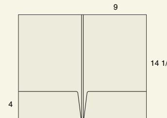
M-118 9 x 14 1/2 Legal size folder with (2) 4" glued pockets and 1/4" spine
