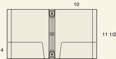
M-702 Binder with (2) 4" glued pockets and reinforced edges (1/2" ring size shown)
