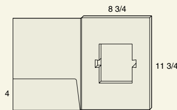
M-613 CD Cavity Box with (1) 4" glued horizontal left pocket. Cavity on right with tray houses 1 CD jewel case. Ships fully assembled. Styrene reinforcement optional.
