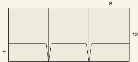
M-400 9 x 12 Folder with (2) 4" outside glued pockets and (1) 4" center unglued flap
