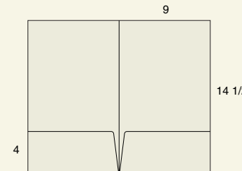
M-116 9 x 14 1/2 Legal size folder with (2) 4" glued pockets
