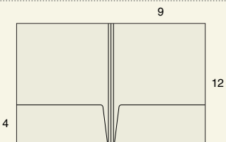
M-111 9 x 12 Folder with (2) 4" glued pockets and triple score spine
