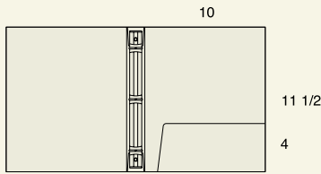
M-701 Binder with (1) 4" glued pocket (1/2" ring size shown)
